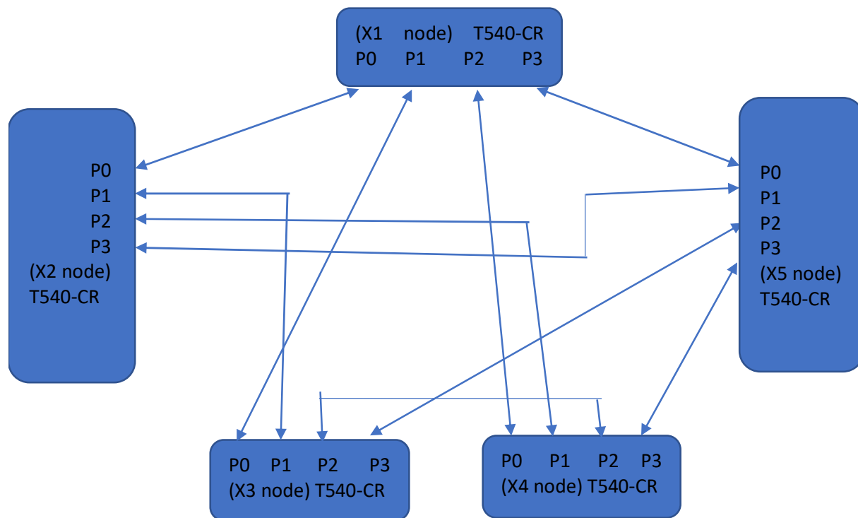
Figure 84 - Mesh Topology
