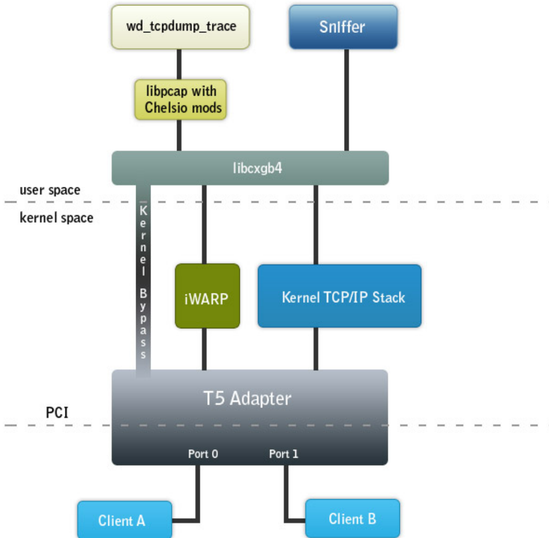
Schematic diagram of sniffer and tracer
